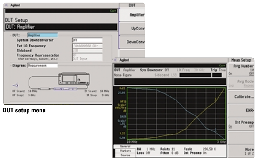
Noise figure and gain measurement
