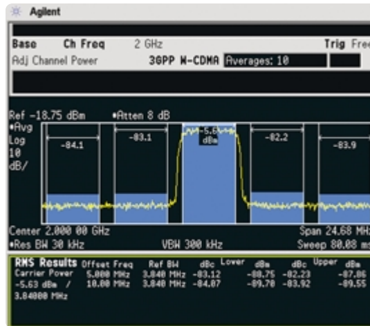
W-CDMA ACP measurement
