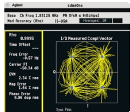
cdmaOne modulation accuracy
