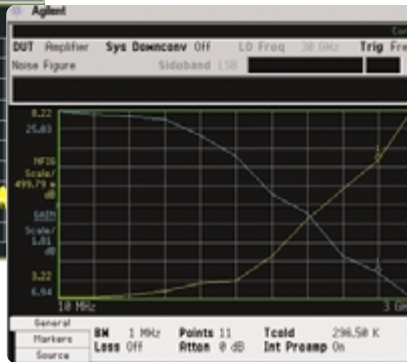
Noise figure and gain measurement
