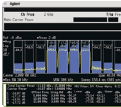
W-CDMA multi-carrier power measurement
