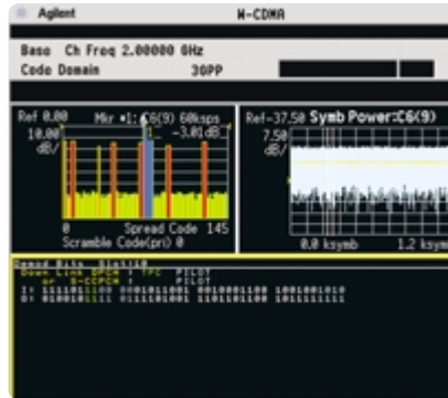
W-CDMA codedomain analysis
