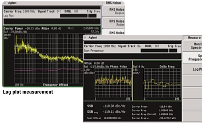
Spot frequency measurement
